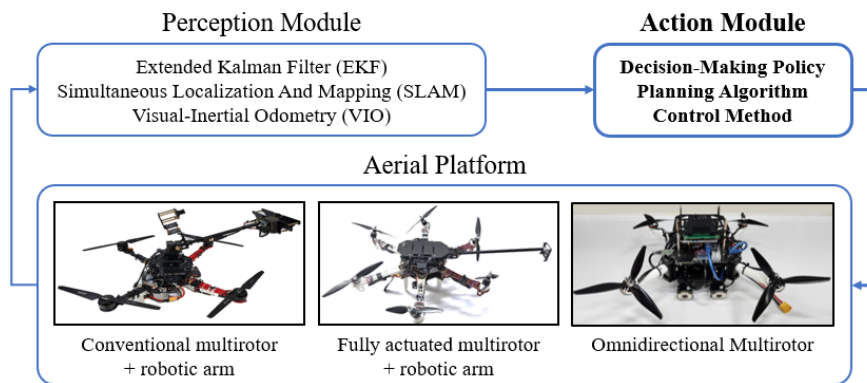
Fig. 1 Structure of fully autonomous aerial manipulation
