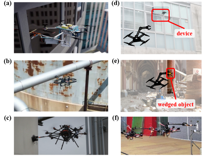
Fig. 1: Types of various APhI tasks. (a) Window-cleaning, (b) Non-Destructive Testing (NDT) on industrial pipes, (c) NDT on industrial walls, (d) Sensor retrieval, (e) Extraction of wedged objects, (f) Plug-pulling.
